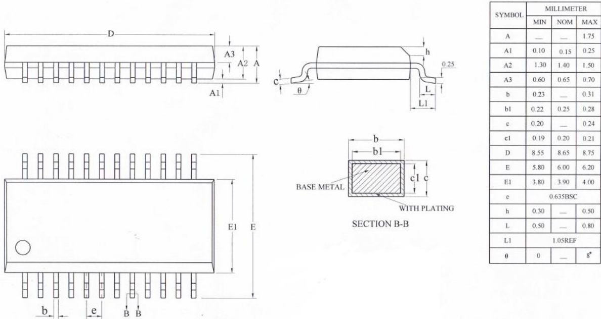
Figure 4-1 AW305A Package
