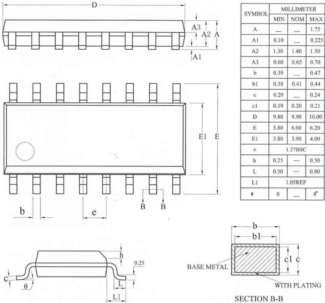
Figure 3-1. AD152A_SOP16 Package
