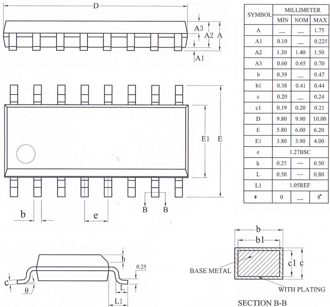
Figure 3-1. AD142A4_SOP16 Package
