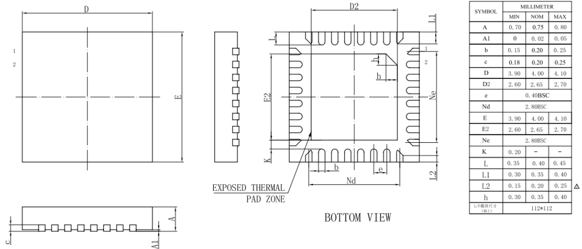
Figure 3-1 AC7006D Package
